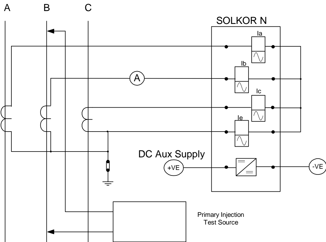
Phase to Phase Primary Injection Test Circuit
